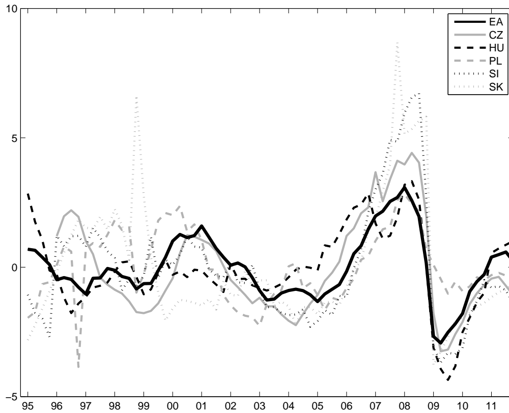
Figure 7: Output
